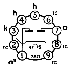
B9A Base
